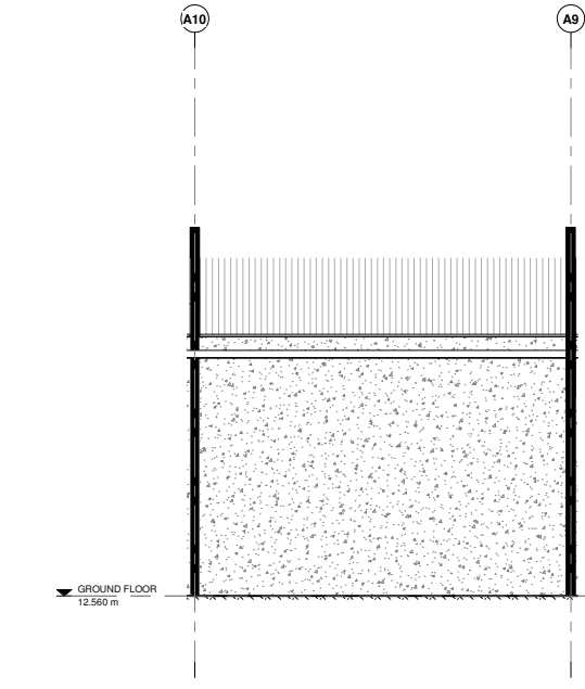
2 Unit Type 01 - Rear Elevation Scale 1:50 @ A1
