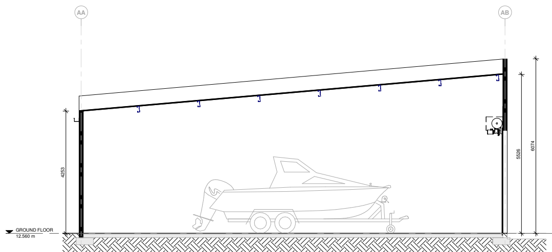
1 Unit Type 01 - Front Elevation Scale 1:50 @ A1
