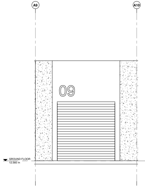
1 Unit Type 01 - Front Elevation Scale 1:50 @ A1
