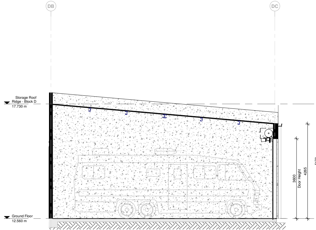
2 Unit Type 04 - Section MA04.01 Scale 1 : 50 @ A1
