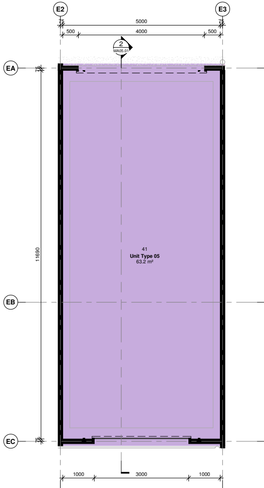
1 Unit Type 05 - Ground Floor Scale 1:50 @ A1
