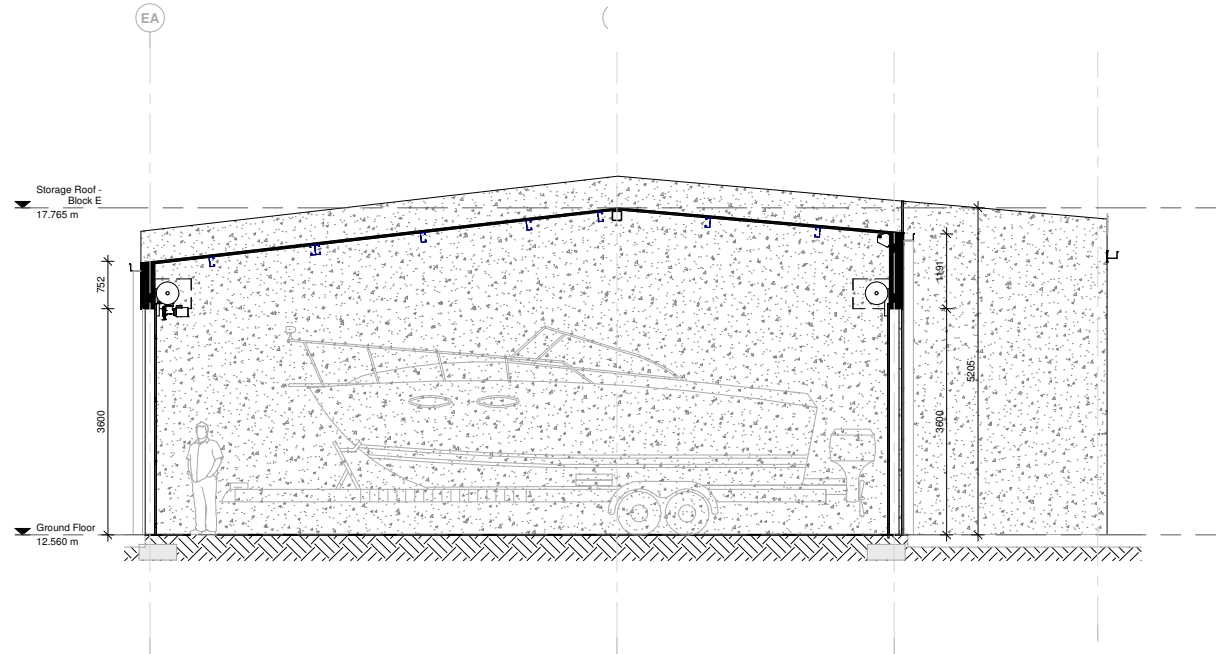
2 Unit Type 05 - Section MA05.01 Scale 1:50 @ A1
