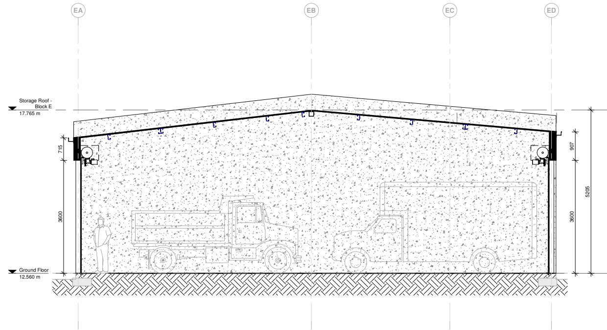
2 Unit Type 06a, 06b - Section MA06.01 Scale 1 : 50 @ A1
