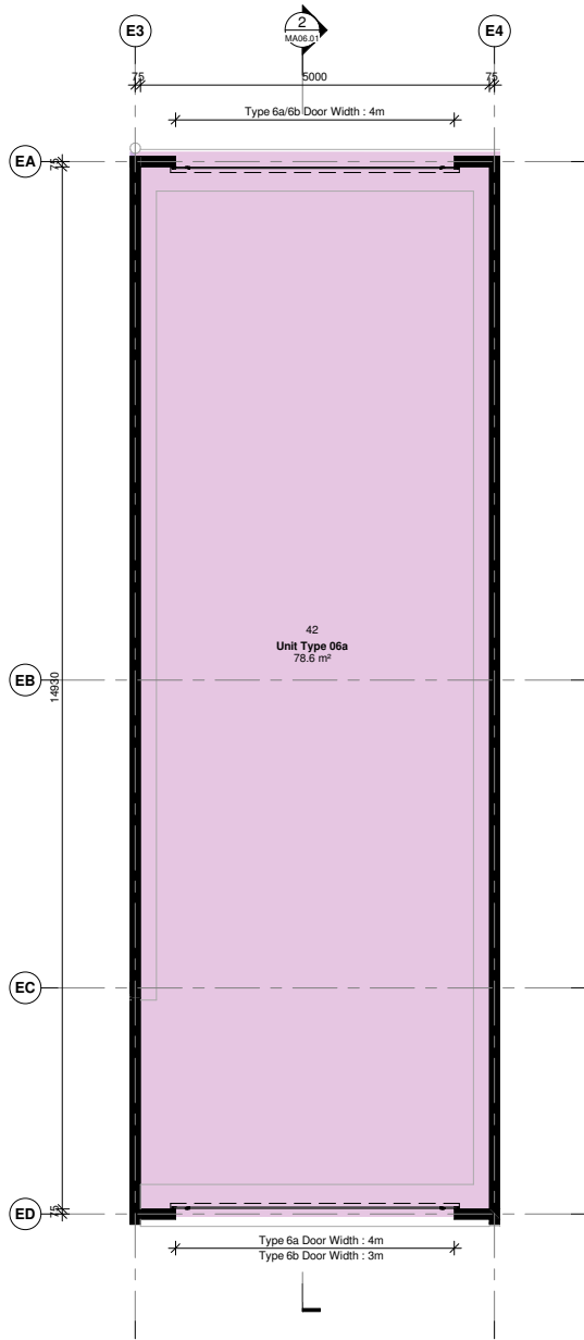
1 Unit Type 06a, 06b - Ground Floor Scale 1 : 50 @ A1
