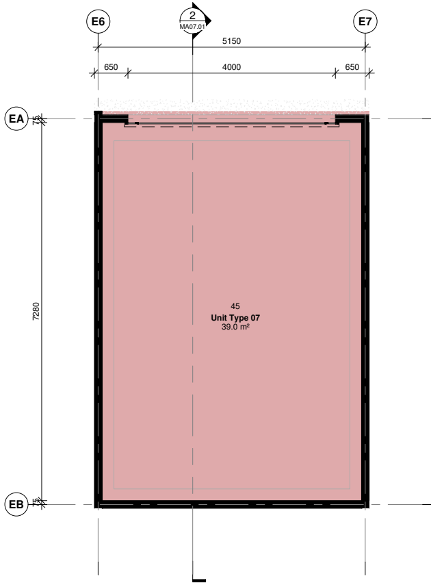
1 Unit Type 07 - Ground Floor Scale 1 : 50 @ A1
