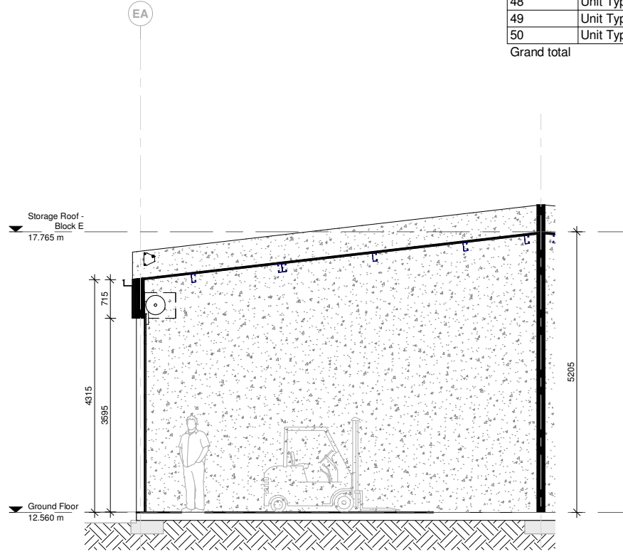
2 Unit Type 07 - Section MA07.01 Scale 1 : 50 @ A1
