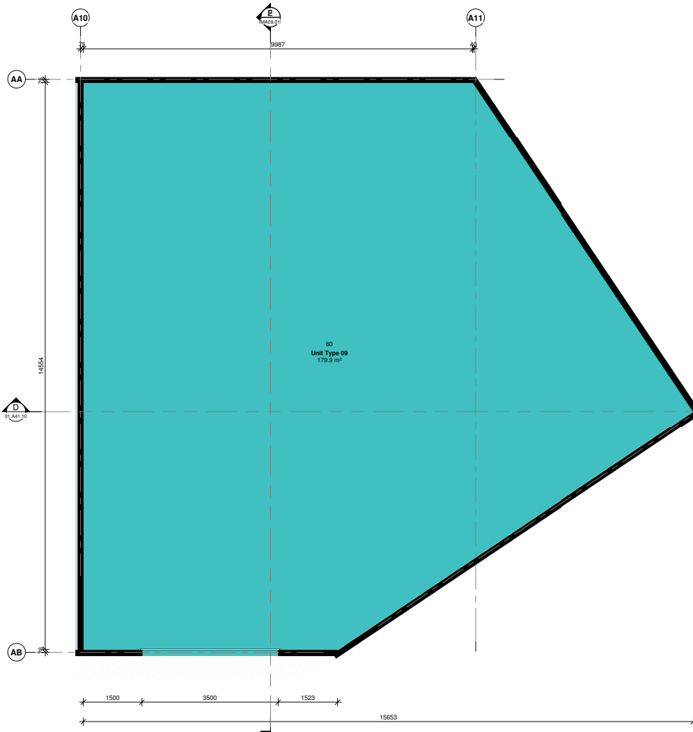
1 Unit Type 09 - Ground Floor Scale 1:50 @ A1
